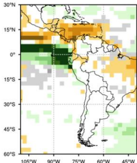
Probabilistic Multi-Model Ensemble Forecast Beijing,CMCC,CPTEC,Melbourne,Monreal,Moscow,Offenbach,Seoul
