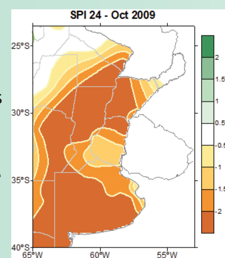
Fig. 3. SPI for 24 - month scale, October 2009.
