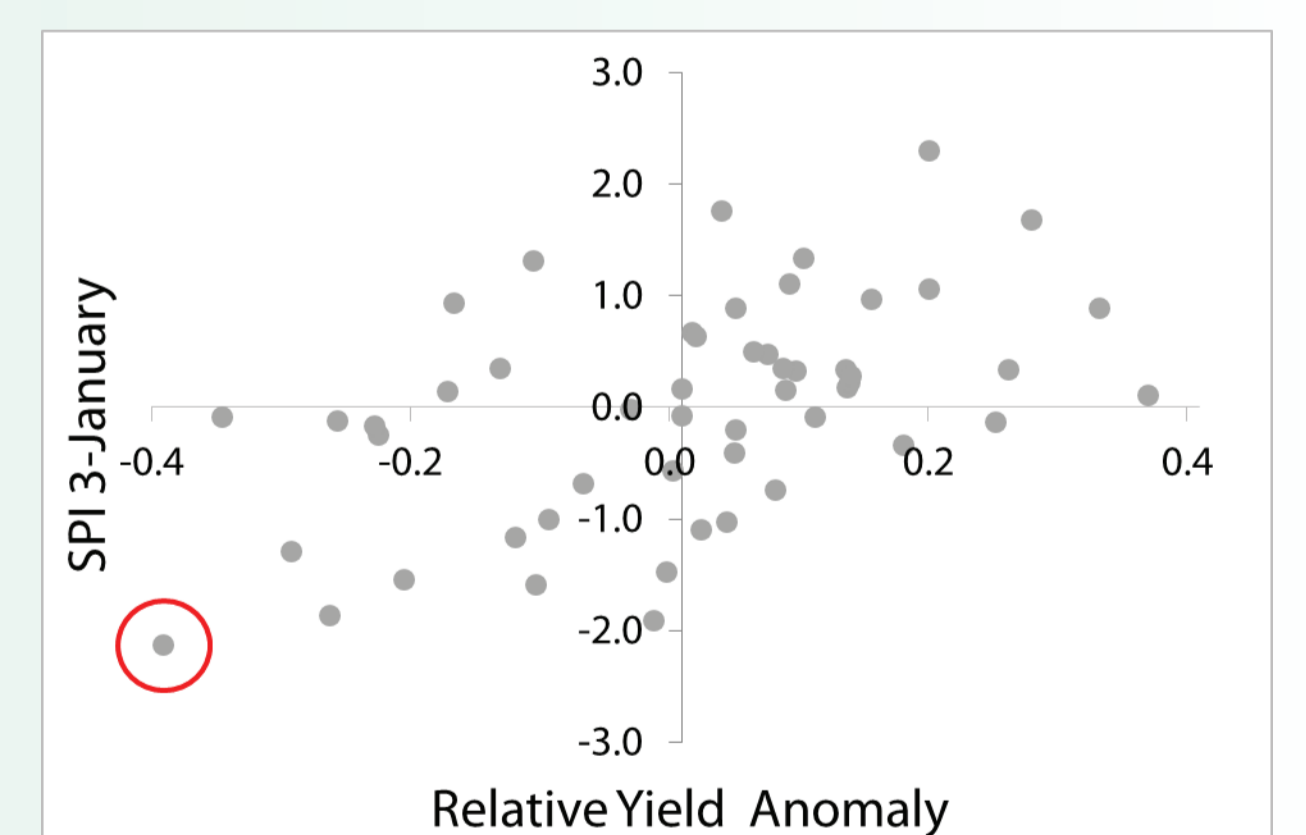
Fig. 7. Junin relative anomaly vs. SPI 3-January.
