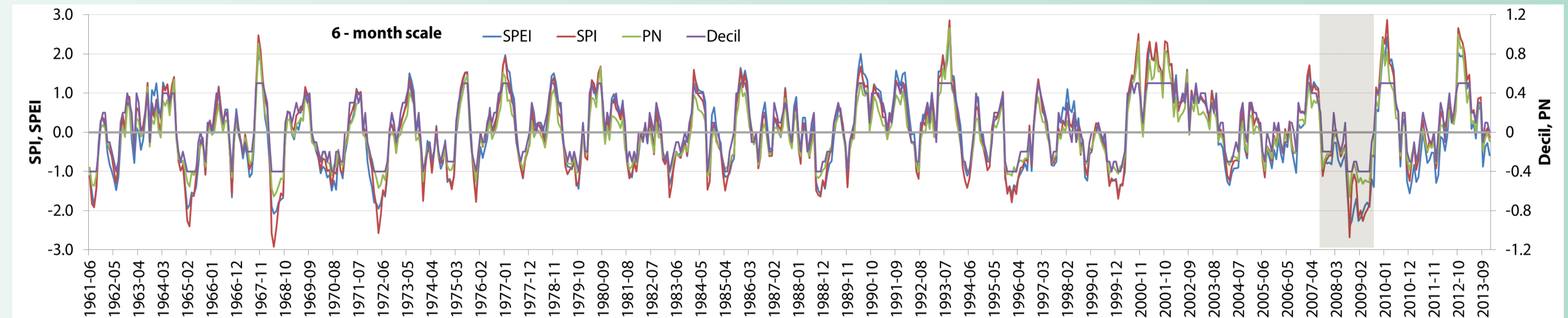
Fig. 1. Junin (E87548) drought indices in 6 - month scale: SPEI, SPI, PN and Decil. Decil and PN were transformed as: [(Decil - 5)/10] and [(PN - 100) / 100] .
